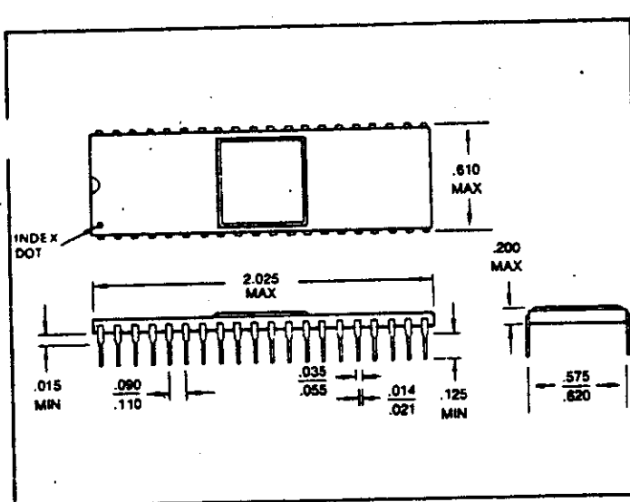
FD179XA-02 CERAMIC PACKAGE
