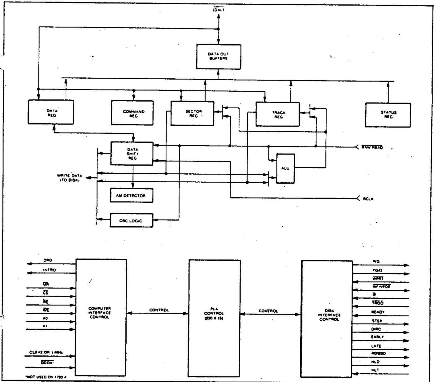
FD179X BLOCK DIAGRAM
