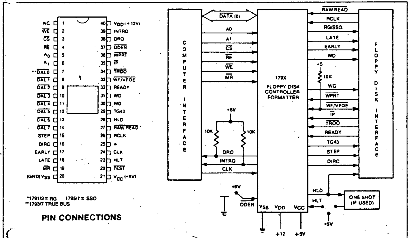
FD179X SYSTEM BLOCK DIAGRAM
