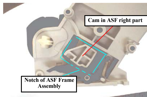
Figure 7-29. ASF Hopper Assembly Cam Matching Position
