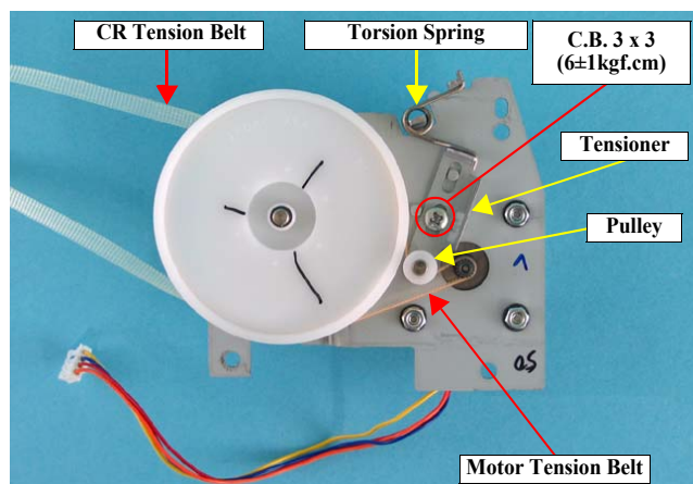
Figure 4-25. Removing the Motor Tension Belt and the CR Tension Belt
