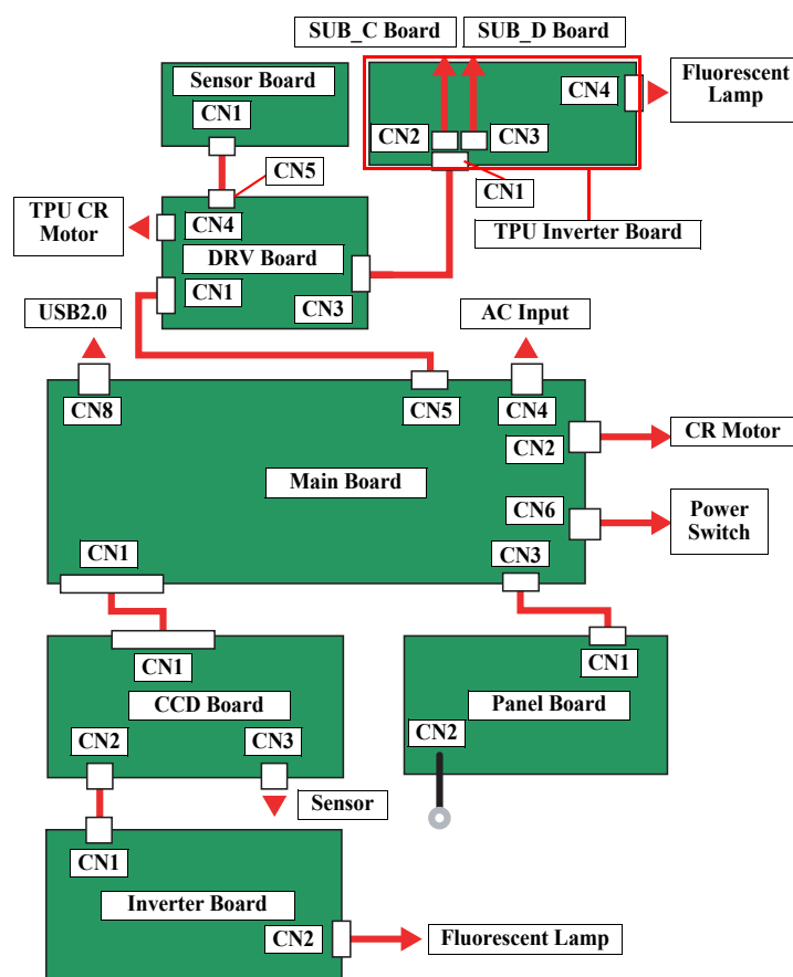
Figure 7-1. Diagram of Wiring Connectors
