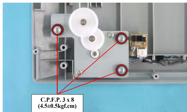
Figure 4-47. Removing the TPU CR Motor Unit (1)
