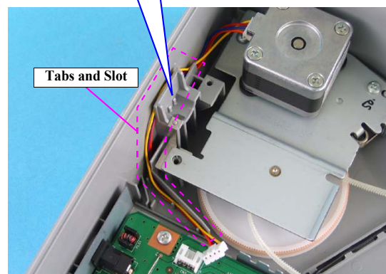
Figure 4-24. Routing the CR Motor Cable
