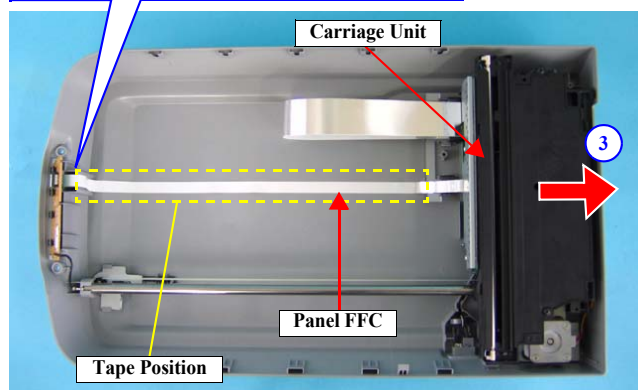
Figure 4-19. Removing the Panel FFC
