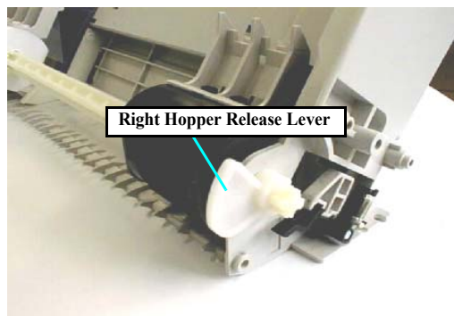
Figure 7-31. Hopper Release Lever Installing Orientation
