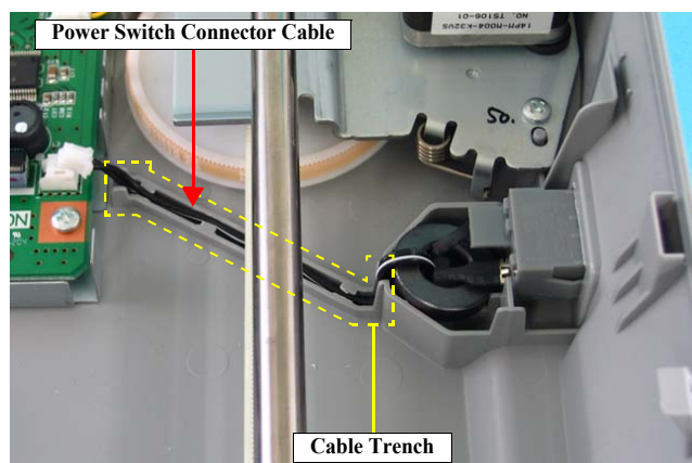
Figure 4-17. Removing the Power Supply Cable Cover
