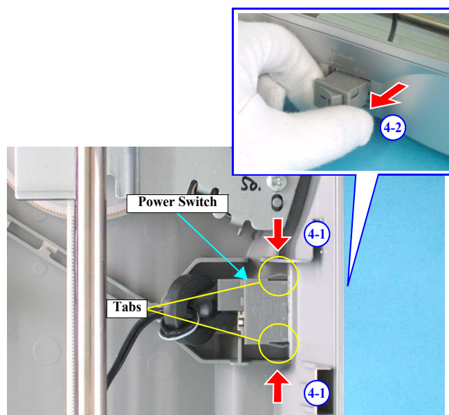
Figure 4-18. Removing the Power Switch
