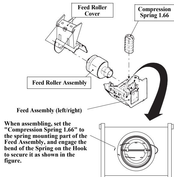
Figure 7-37. Disassembly of Feed Roller Assembly
