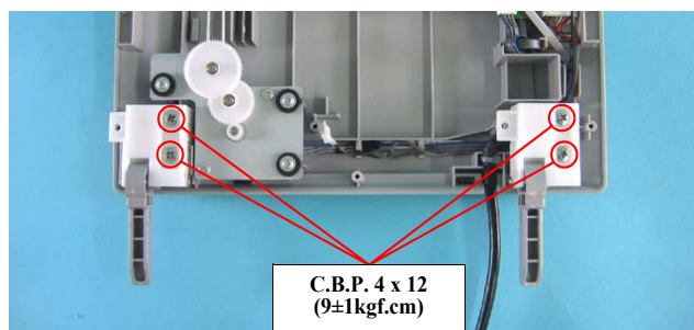
Figure 4-30. Removing the Hinge Assy.
