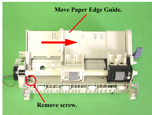
Figure 7-21. Disassembly of ASF and Frame 1
