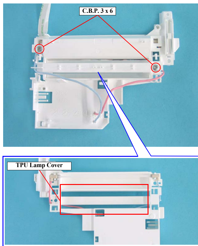
Figure 4-43. Removing the TPU Lamp Cover
