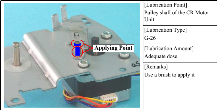
Figure 6-1. Lubricating the CR moter Unit
