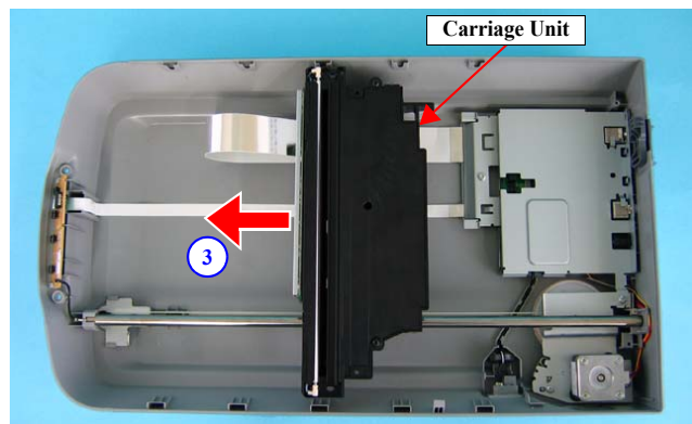
Figure 4-6. Moving the Carriage Unit
