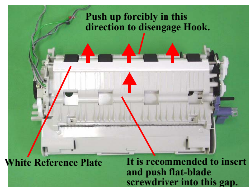
Figure 7-16. White Reference Plate Removal 1
