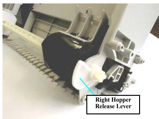
Figure 7-25. Removal of Right Hopper Release Lever
