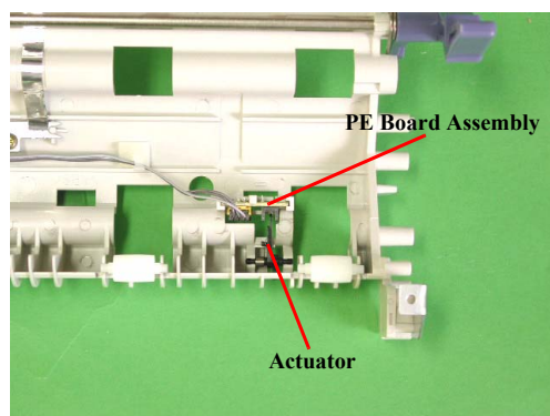
Figure 7-24. Removal of Actuator and PE Board Assembly 2
