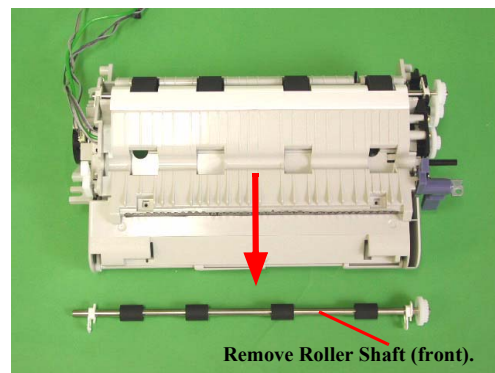
Figure 7-15. Roller Removal 2
