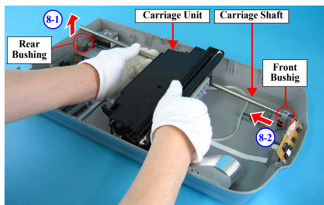
Figure 4-9. Removing the Carriage Shaft
