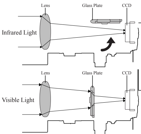
Figure 2-7. Refraction of Infrared Light and Visible Light
