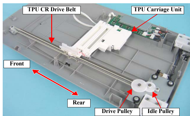
Figure 2-6. TPU Carriage Operation
