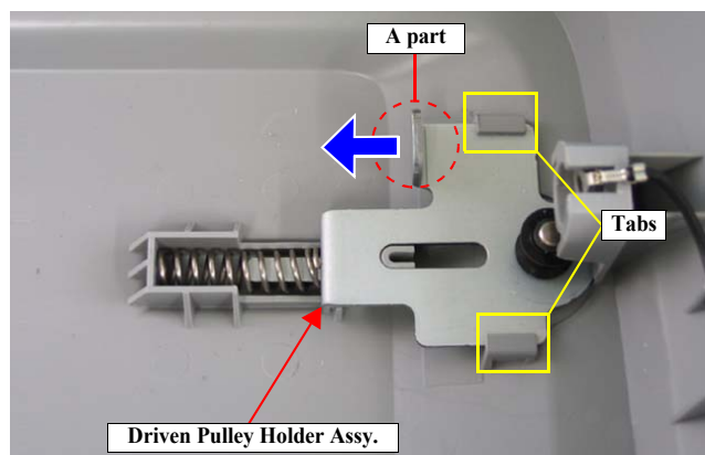
Figure 4-21. Removing the Driven Pulley Holder Assy.
