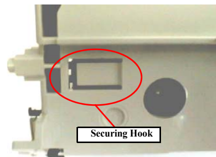
Figure 7-34. Right Feed Roller Assembly Securing Hook Position
