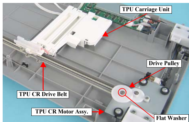
Figure 4-36. Removing the TPU CR Drive Belt
