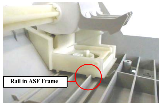
Figure 7-32. Feed Roller Assembly Installation Point
