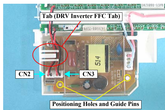
Figure 4-41. Routing the DRV Inverter Cables
