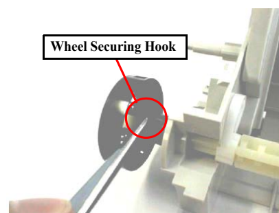
Figure 7-27. Removal of ASF HP Detection Wheel
