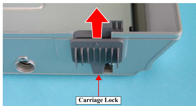
Figure 4-12. Removing the Carriage Lock
