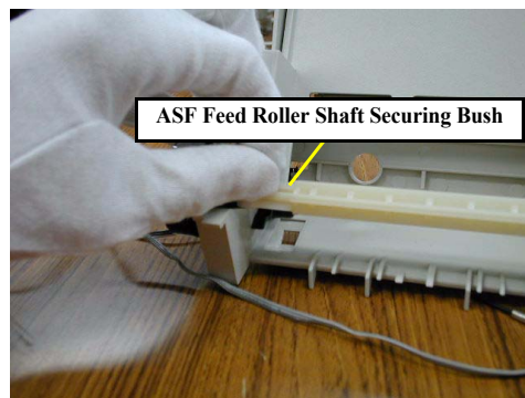
Figure 7-26. Removal of ASF Feed Roller Securing Bush
