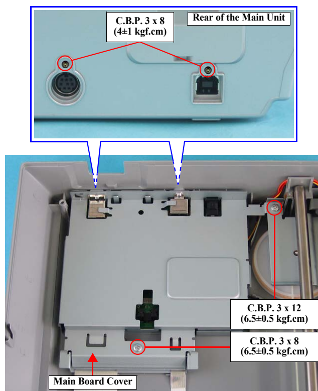
Figure 4-13. Removing the Main Board Cover (1)
