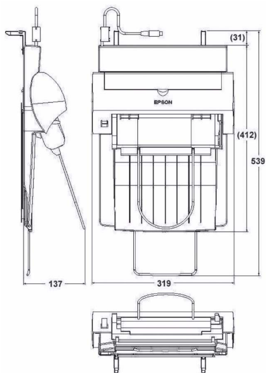
Figure 7-2. ADF Overview Drawing
