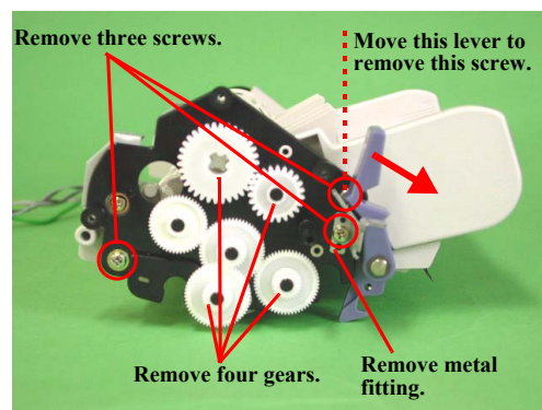
Figure 7-19. Gear Removal
