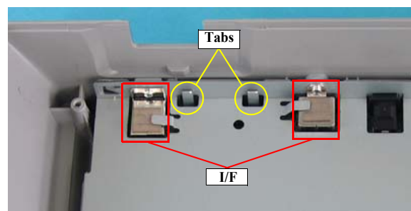
Figure 4-15. Installing the Main Board Cover
