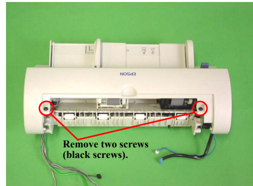
Figure 7-9. Screw Removal
