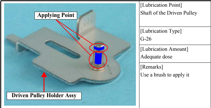
Figure 6-2. Lubricating the Driven Pulley Holder Assy
