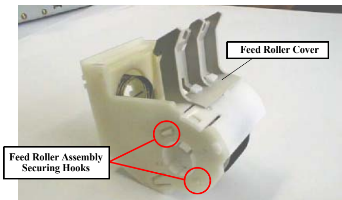
Figure 7-36. Feed Roller Assembly Removal Hook Position
