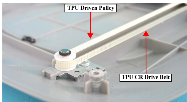
Figure 4-48. Removing the TPU CR Motor Unit (2)
