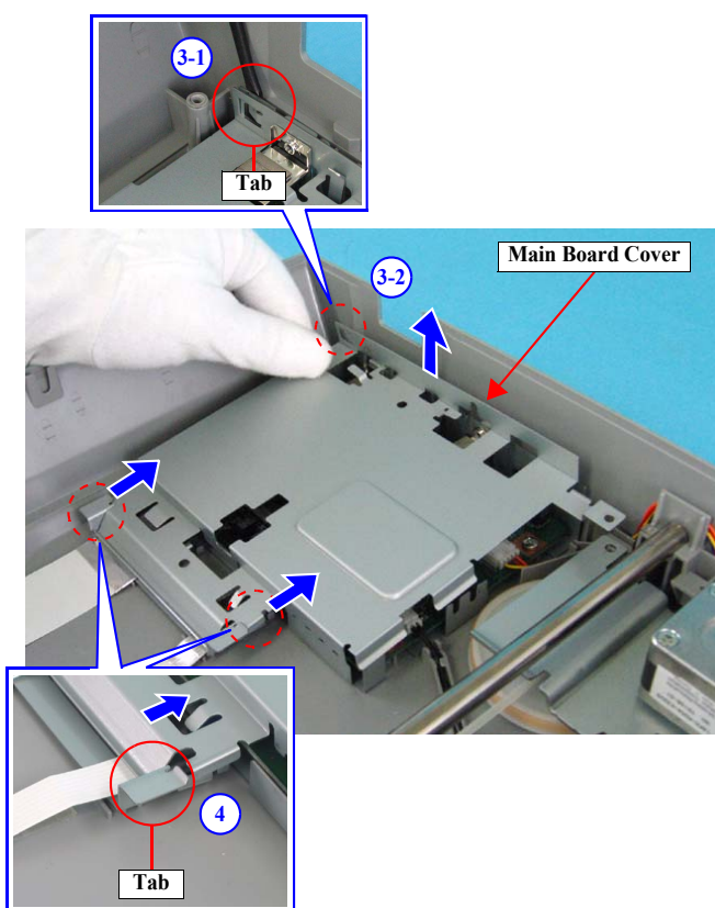
Figure 4-14. Removing the Main Board Cover (2)
