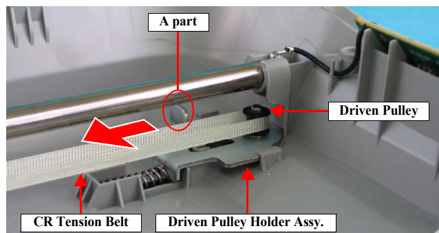
Figure 4-8. Removing the CR Tension Belt
