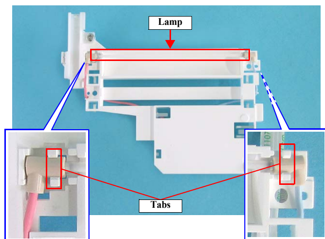
Figure 4-44. Removing the Lamp
