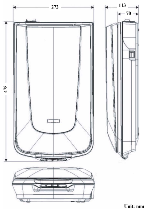
Figure 1-3. External Dimensions of Perfection 4490 Photo
