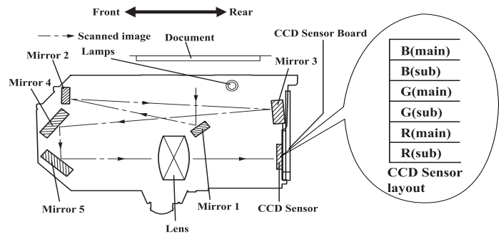
Figure 2-2. Mirror/Lens Mechanism
