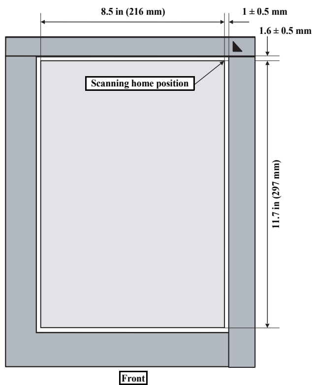
Figure 1-4. Reflective Document Scanning Range
