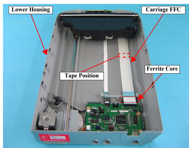
Figure 4-7. Removing the Carriage FFC
