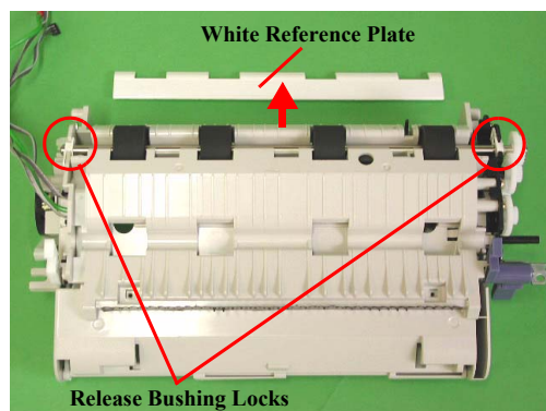
Figure 7-17. White Reference Plate Removal 2
