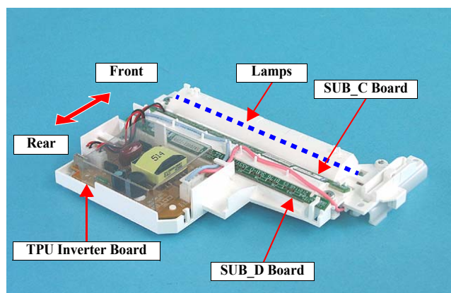
Figure 2-3. TPU Carriage Unit Configuration
