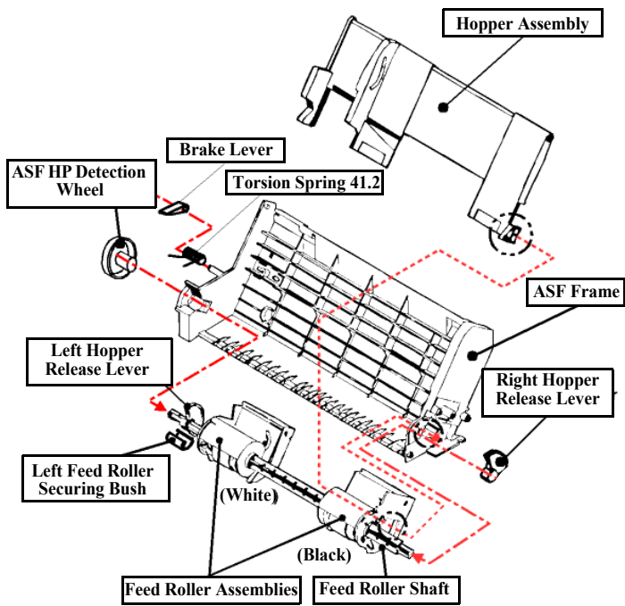
Figure 7-30. Disassembly of ASF Assembly
