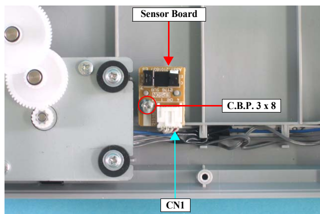
Figure 4-29. Removing the Sensor Board
