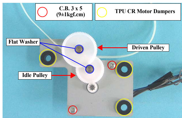
Figure 4-49. Removing the TPU CR Motor Dampers and TPU CR Motor
