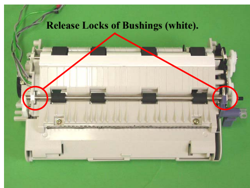
Figure 7-14. Roller Removal 1
