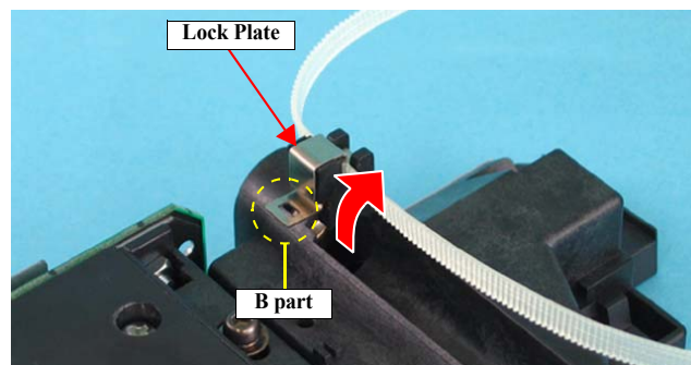
Figure 4-10. Removing the Carriage Unit
