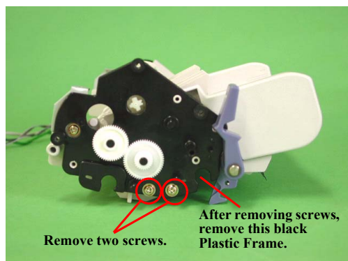
Figure 7-20. Removal of Plastic Frame
