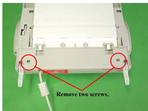
Figure 7-4. ADF Rear Screw Removal
