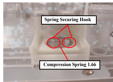
Figure 7-35. Compression Spring 1.66 Temporarily Securing Position
