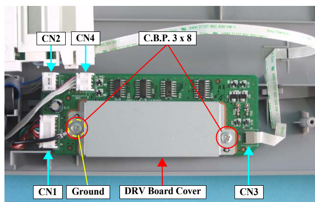
Figure 4-33. Removing the DRV Board (1)
