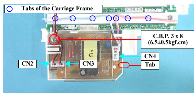
Figure 4-39. Removing the TPU Inverter Board (1)
