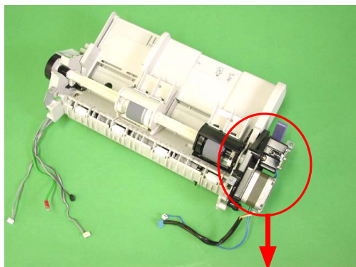
Figure 7-11. Removal of Motor/Solenoid Assembly
