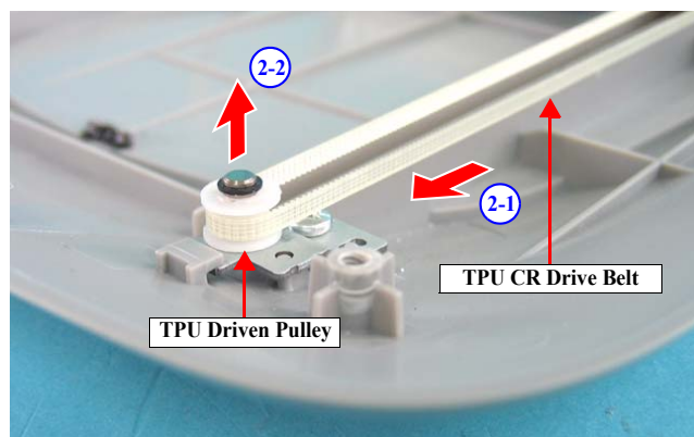
Figure 4-34. Removing the TPU CR Drive Belt (2)
