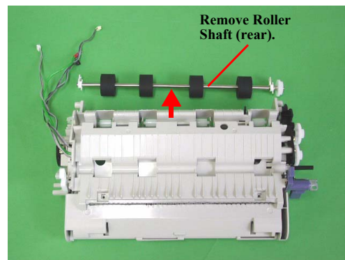
Figure 7-18. Roller Removal
