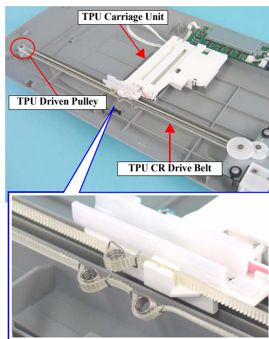
Figure 4-35. Installing the Torsion Springs
