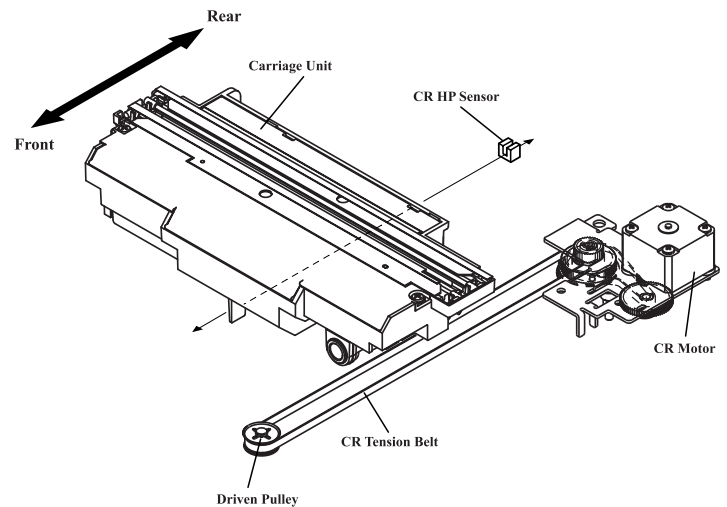
Figure 2-5. Carriage Operation
