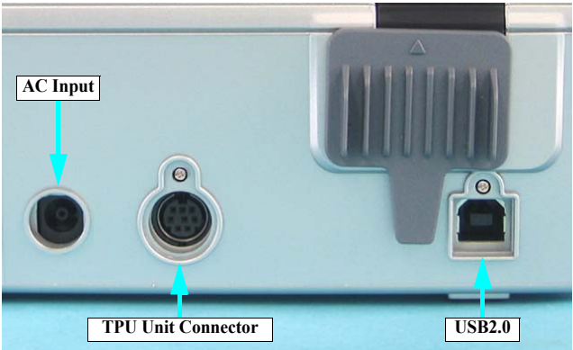
Figure 1-1. Interface
