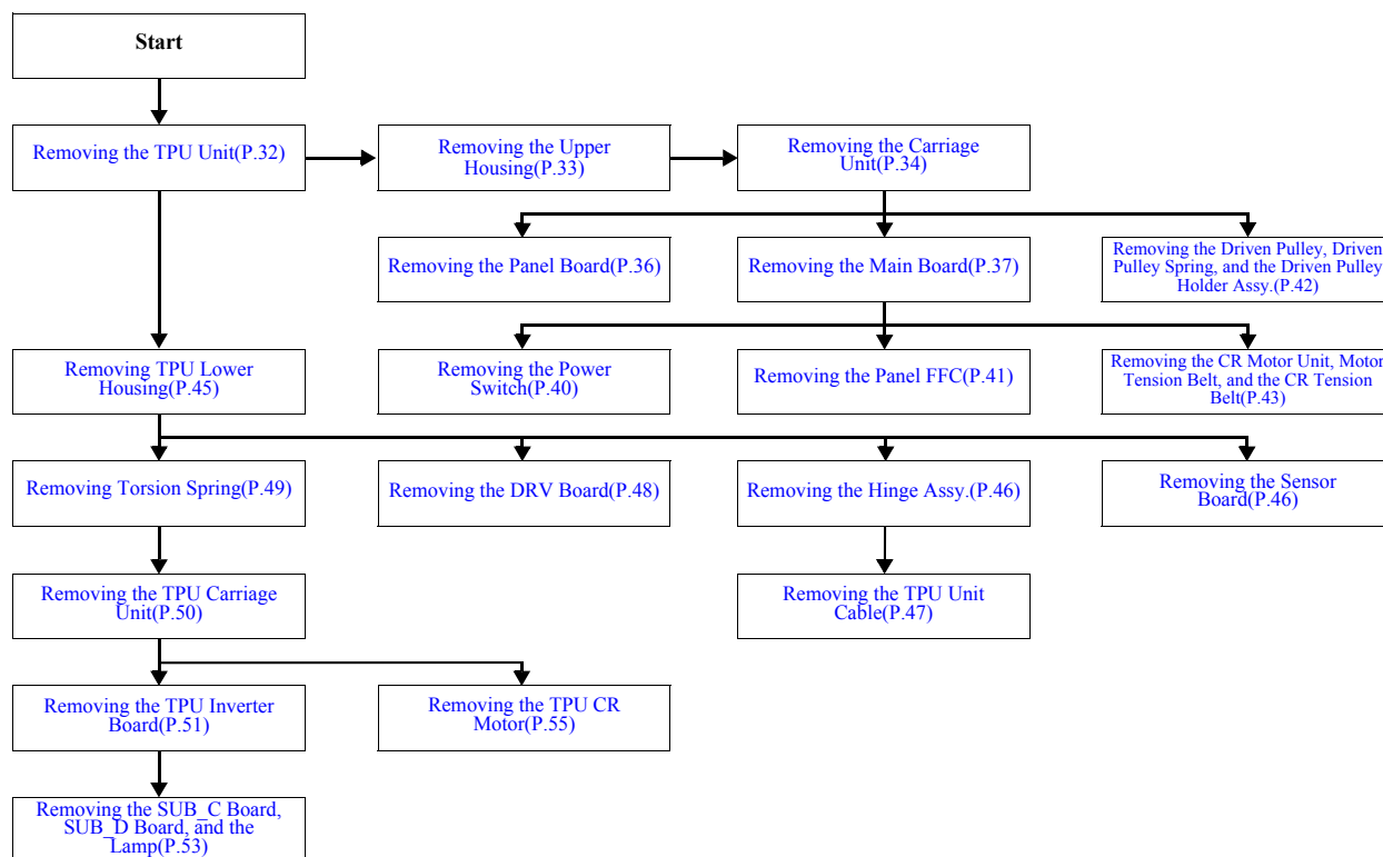
Figure 4-1. Disassembly Flowchart
