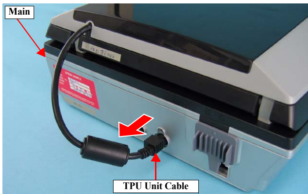
Figure 4-2. Removing the TPU Unit (1)
