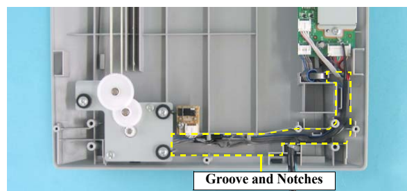
Figure 4-50. Routing the TPU CR Motor Cables
