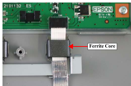
Figure 4-20. Installing the Ferrite Core
