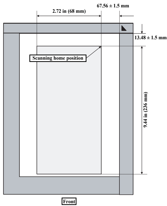
Figure 1-5. Transparent Document Scanning Range
