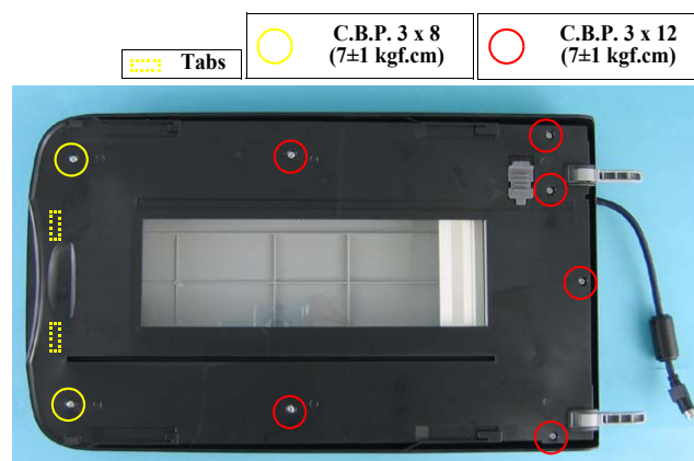
Figure 4-27. Removing the TPU Lower Housing (1)
