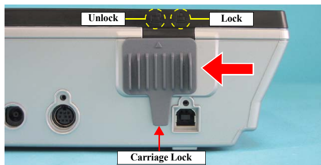
Figure 4-5. Releasing the Carriage Lock
