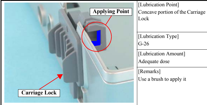
Figure 6-3. Lubricating the Carriage Lock
