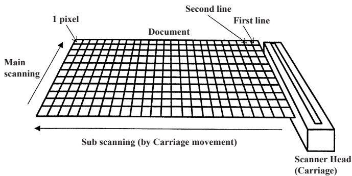
Figure 2-4. Carriage Movement
