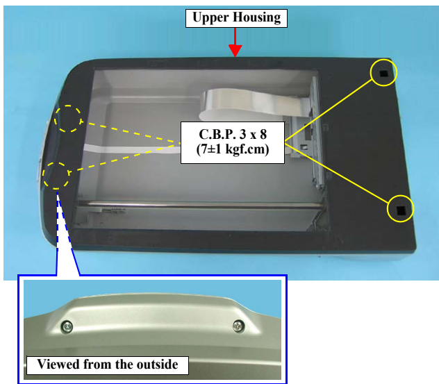
Figure 4-4. Removing the Upper Housing
