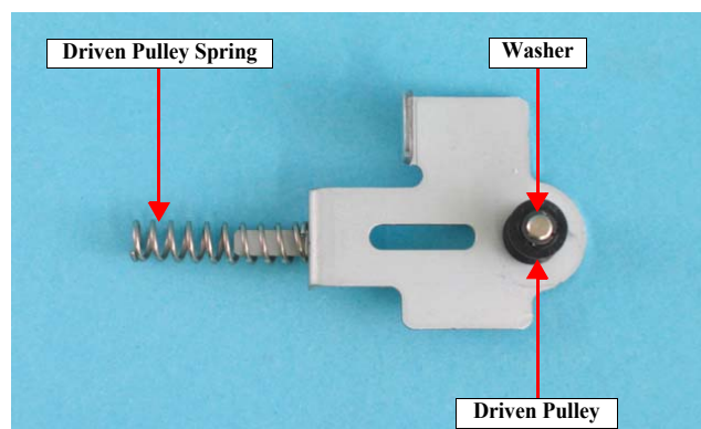
Figure 4-22. Removing the Driven Pulley and the Driven Pulley Spring
