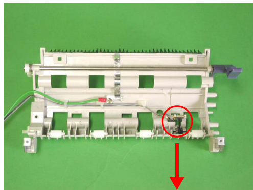
Figure 7-23. Removal of Actuator and PE Board Assembly 1
