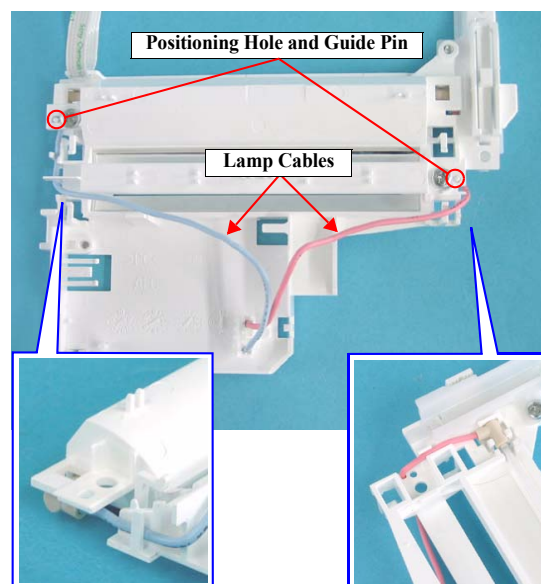
Figure 4-45. Routing the Lamp Cables
