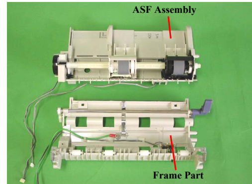
Figure 7-22. Disassembly of ASF and Frame 2
