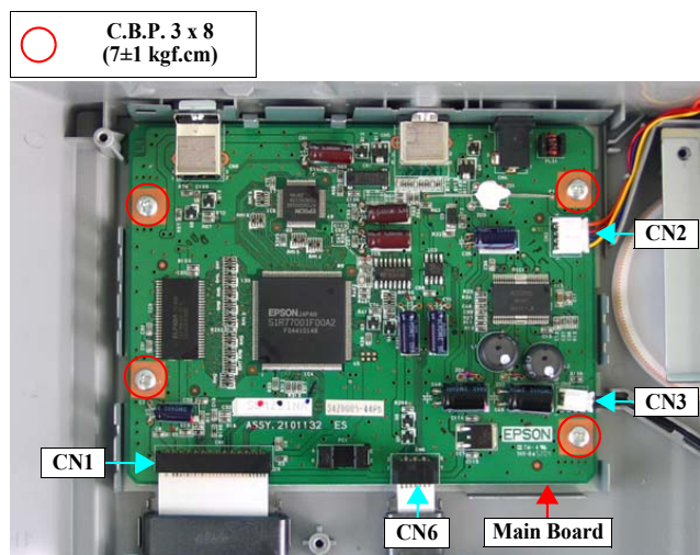
Figure 4-16. Removing the Main Board
