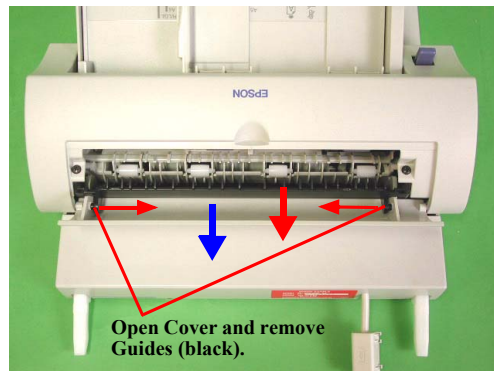
Figure 7-7. Guide Removal
