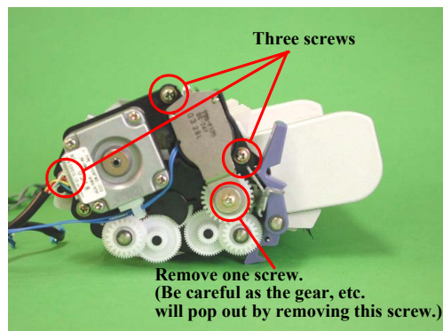
Figure 7-12. Removal of Motor/Solenoid Assembly
