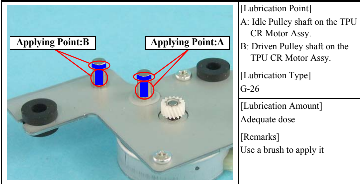
Figure 6-4. Lubricating the TPU CR Moter Assy
