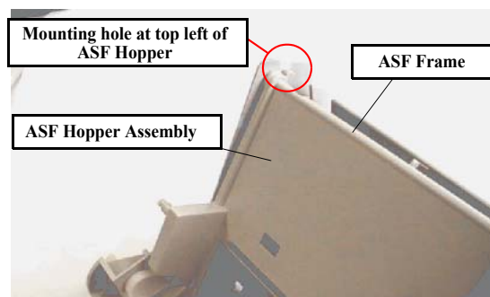
Figure 7-28. ASF Hopper Assembly Removal
