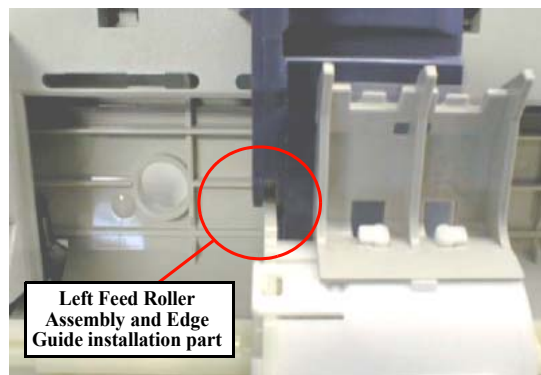
Figure 7-33. Left Feed Roller Assembly Installation Point
