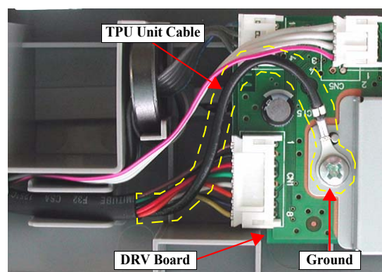
Figure 4-32. Routing the TPU Unit Cable
