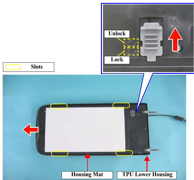
Figure 4-26. Removing the Housing Mat (Document Cover)
