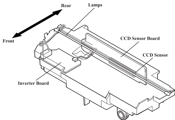
Figure 2-1. Carriage Unit Configuration
