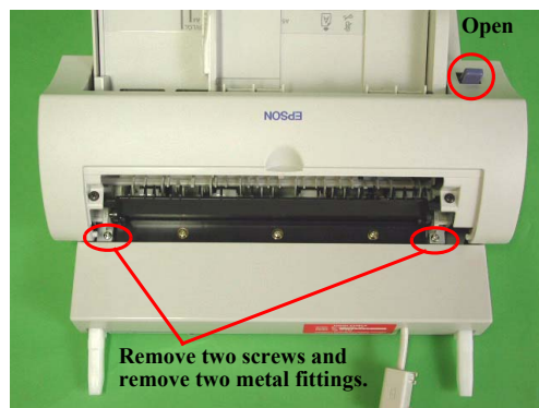
Figure 7-8. Screw and Metal Fitting Removal
