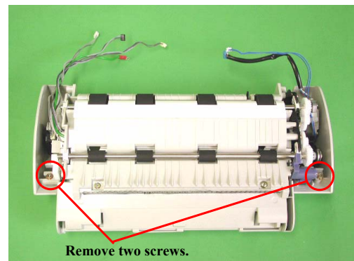
Figure 7-10. Screw Removal
