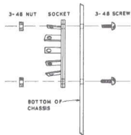
7 & 9 PIN SOCKET MOUNTING
